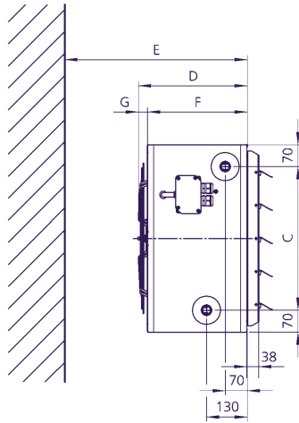
Wandmontage
